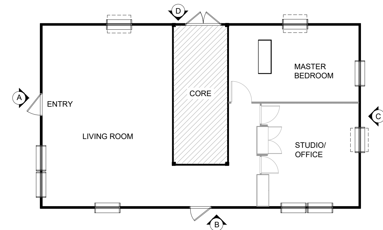
1 OPTION 1 SCALE 1" = 8'-0"
