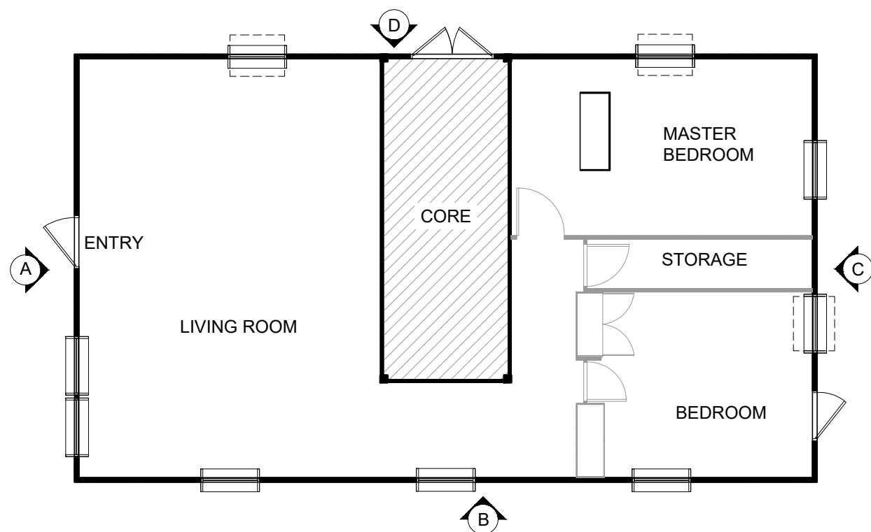
2 OPTION 2 SCALE 1" = 8'-0"
